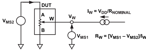
Figure 24. Wiper Resistance
