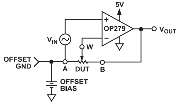
Figure 27. Noninverting Gain
