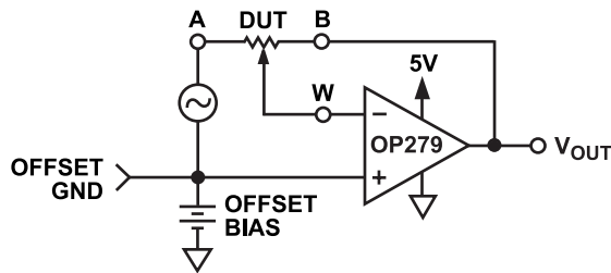
Figure 26. Inverting Gain
