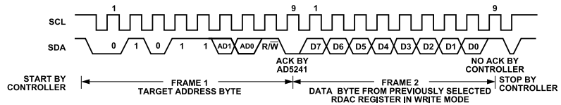
Figure 5. Reading Data from a Previously Selected RDAC Register in Write Mode
