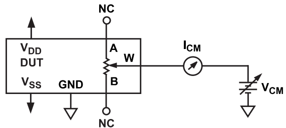
Figure 30. Common-Mode Leakage Current
