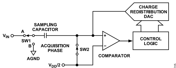
Figure 40. ADC Acquisition Phase
