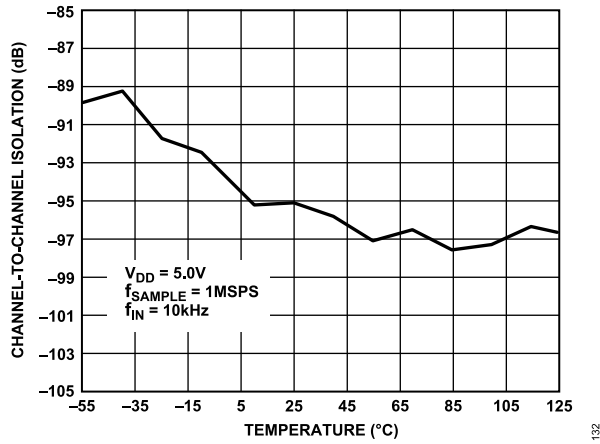
Figure 36. Channel-to-Channel Isolation vs. Temperature
