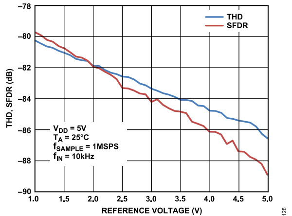
Figure 22. THD and SFDR vs. Reference Voltage
