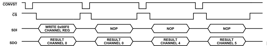
Figure 55. Channel Sequencer
