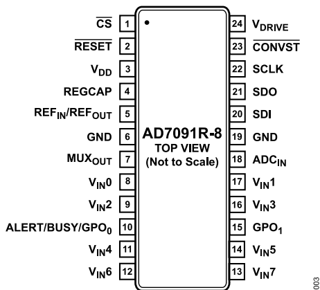
Figure 9. 8-Channel, 24-Lead TSSOP Pin Configuration
