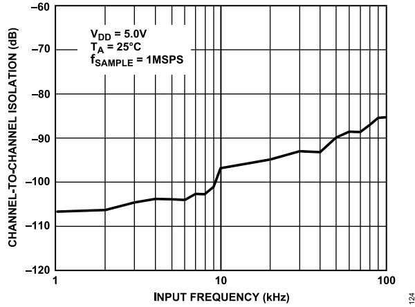
Figure 35. Channel-to-Channel Isolation vs. Input Frequency
