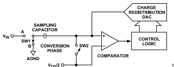
Figure 41. ADC Conversion Phase
