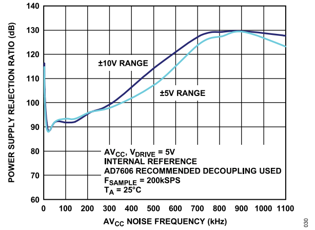
Figure 33. PSRR
