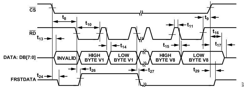
Figure 7. BYTE Mode Read Operation
