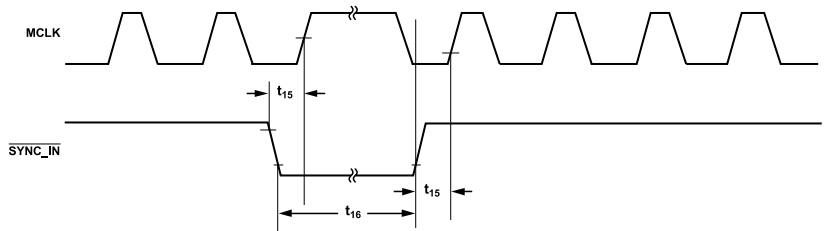
Figure 7. Synchronous \overline{SYNC\_IN} Pulse
