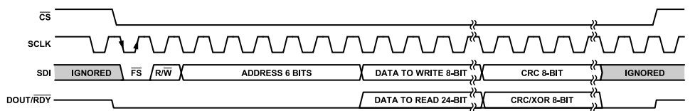
Figure 89. Data Output Format When Using CRC
