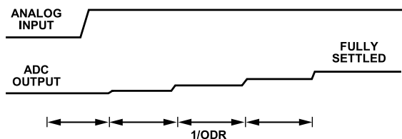
Figure 70. Sinc5 Filter Step Response
