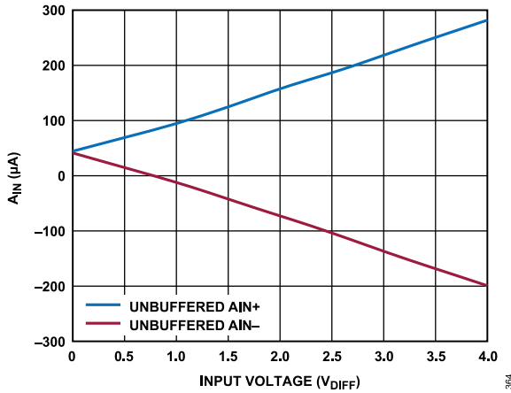
Figure 64. Analog Input Current ( A_{IN} ) vs. Input Voltage, Analog Input Precharge Buffer Off, V_{CM} = 2.5\text{ V} , f_{MOD} = 8.192\text{ MHz}
