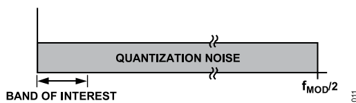
Figure 57. \Sigma - \Delta ADC Quantization Noise (Linear Scale X-Axis)
