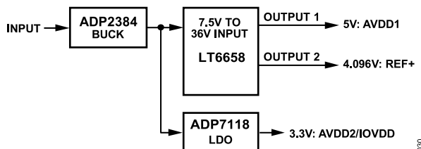
Figure 80. LT6658 Used as Both an AVDD1 Supply and Reference
