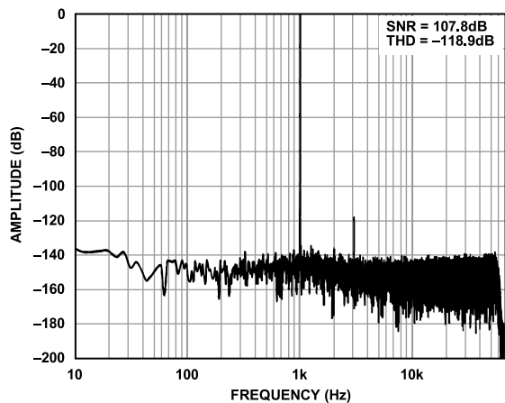
Figure 11. FFT, Median Mode, Low Ripple FIR Filter, -0.25 dBFS
