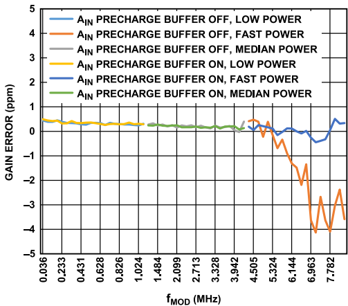
Figure 36. Gain Error vs. f_{MOD}
