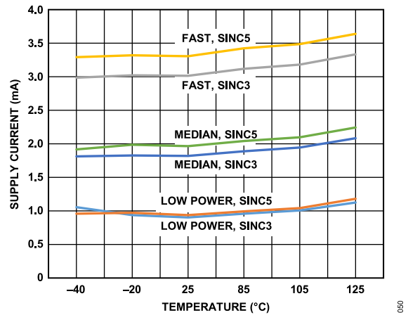
Figure 50. Supply Current vs. Temperature, IOVDD, Sinc3 and Sinc5 Filter
