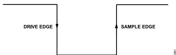
Figure 85. SPI Mode 3
