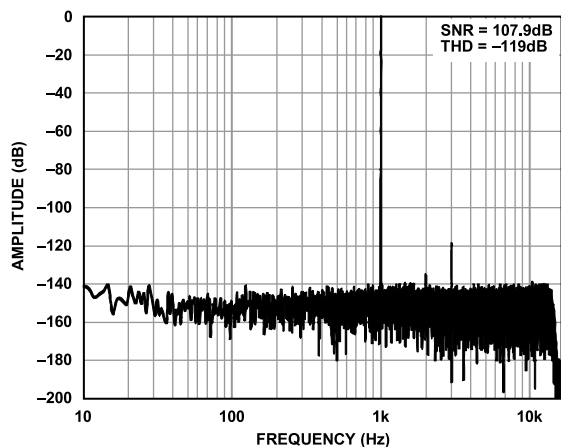
Figure 12. FFT, Low Power Mode, Low Ripple FIR Filter, -0.25 dBFS
