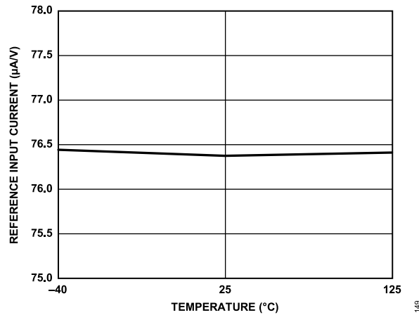
Figure 47. Reference Input Current vs. Temperature, Reference Precharge Buffers Off
