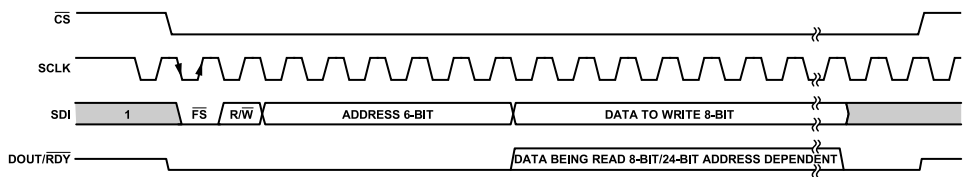
Figure 86. SPI Basic Read/Write Frame
