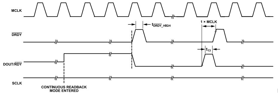
Figure 6. DOUT/\overline{RDY} Behavior Without SCLK Applied
