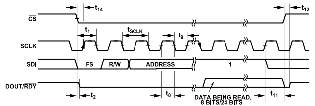
Figure 2. SPI Read Timing Diagram
