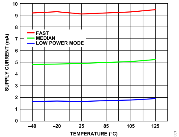
Figure 51. Supply Current vs. Temperature, IOVDD, Low Ripple FIR Filter
