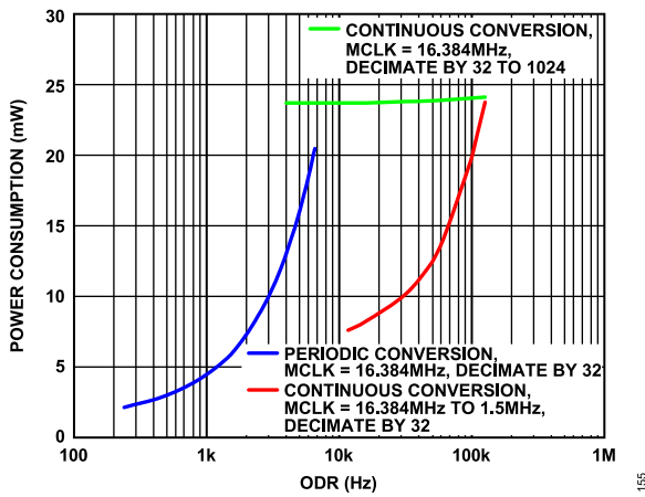
Figure 53. Power Consumption, Conversion Modes vs. ODR, Median Power Mode, Sinc5 Filter
