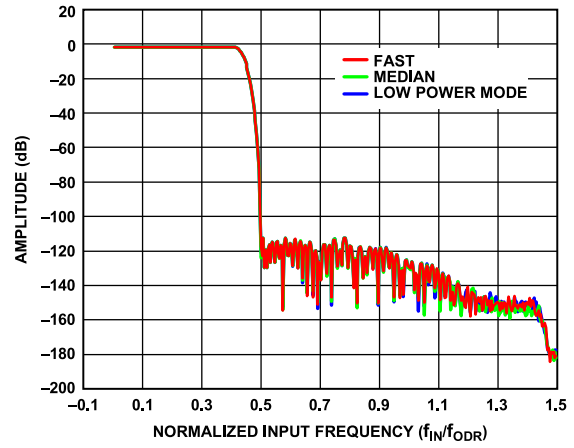
Figure 37. Low Ripple FIR Filter Profile, Amplitude vs. Normalized Input Frequency ( f_{IN}/f_{ODR} )
