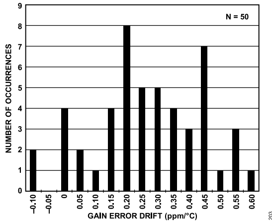
Figure 35. Gain Error Drift Reference Buffers Off
