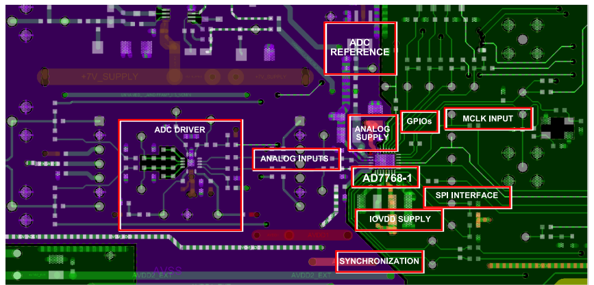
Figure 100. Subsystem Layout
