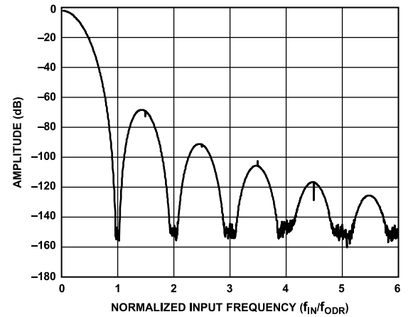
Figure 38. Sinc5 Filter Profile, Amplitude vs. Normalized Input Frequency ( f_{IN}/f_{ODR} )
