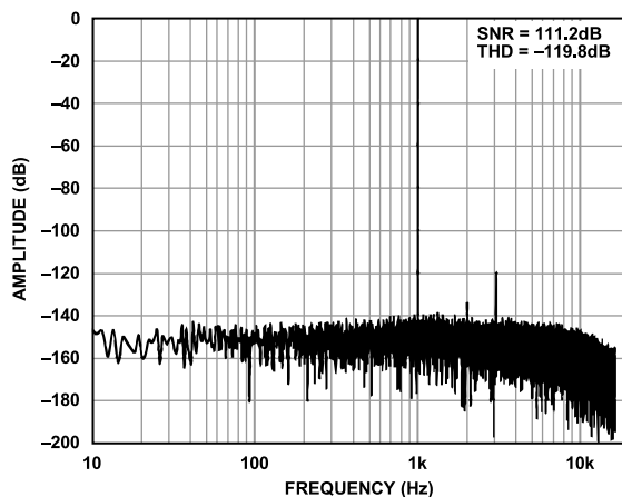
Figure 15. FFT, Low Power Mode, Sinc5 Filter, -0.25 dBFS
