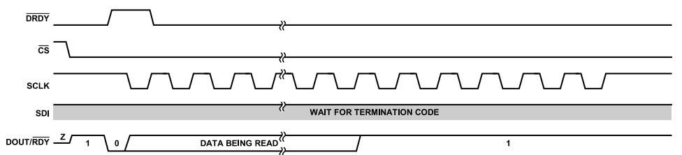
Figure 92. Continuous ADC Read Data Format with \overline{\text{RDY}} Function Enabled on the DOUT/ \overline{\text{RDY}} Pin
