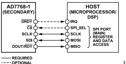
Figure 84. Basic Serial Port Connection Diagram
