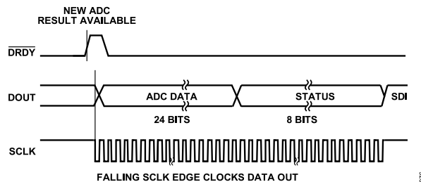
Figure 81. \overline{\text{PIN}} Mode Data Output Format (This Figure Does Not Show the \overline{\text{CS}} Signal)
