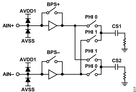
Figure 63. Analog Front End of the AD7768-1
