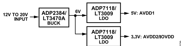
Figure 79. Power Supply Configuration
