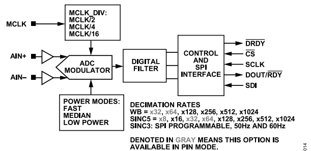
Figure 60. Sampling Structure Defined by the MCLK and MCLK_DIV Settings
