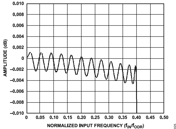
Figure 74. Low Ripple FIR Filter Pass-Band Ripple
