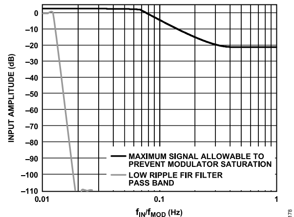
Figure 76. Modulator Saturation Area
