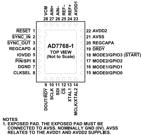
Figure 9. Pin Configuration
