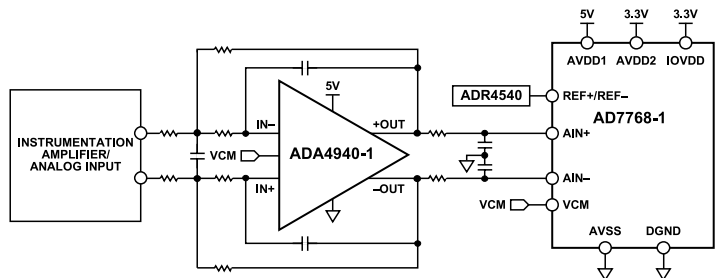
Figure 97. Implementation of a Multiple Feedback, Low-Pass Filter
