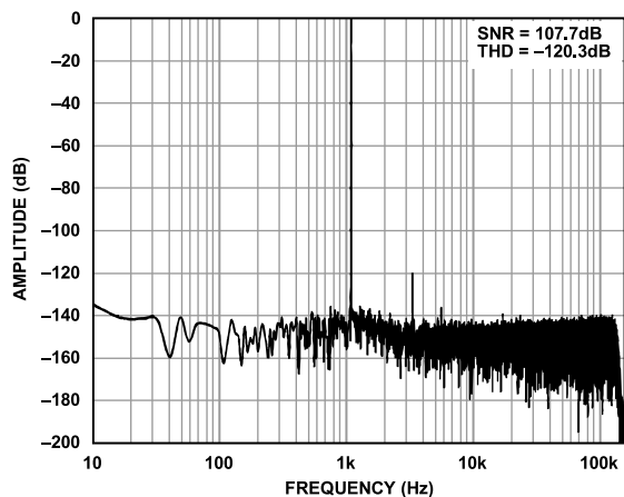
Figure 10. FFT, Fast Mode, Low Ripple FIR Filter, -0.25 dBFS
