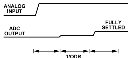
Figure 71. Sinc3 Filter Step Response
