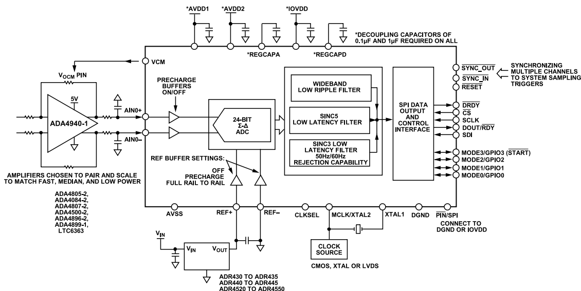
Figure 78. Typical Connection Diagram
