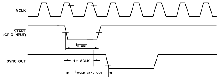
Figure 8. Asynchronous \overline{START} and \overline{SYNC\_OUT}
