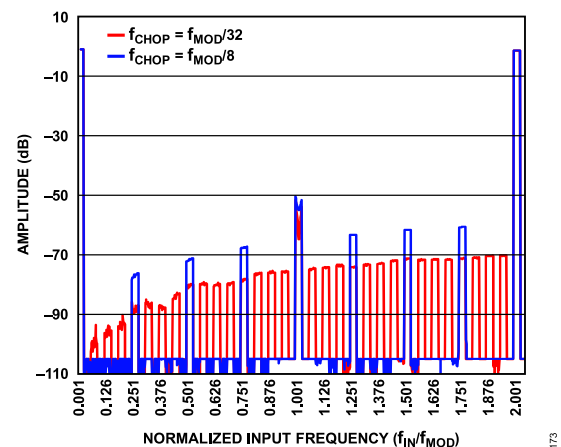
Figure 77. Rejection of Out of Band Tones
