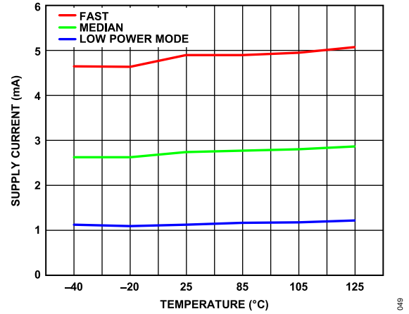
Figure 49. Supply Current vs. Temperature, AVDD2
