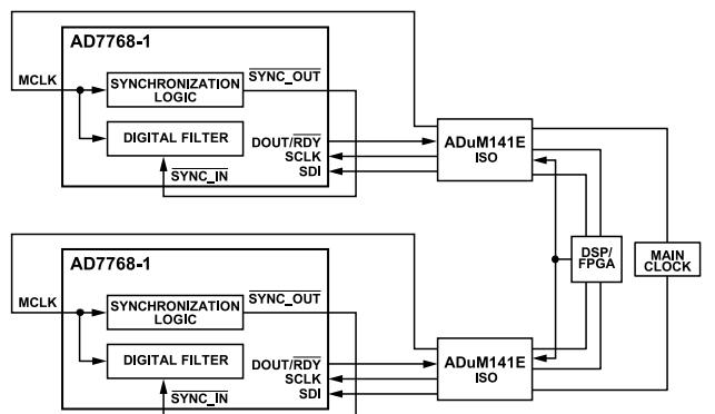
Figure 95. Synchronization in Channel to Channel Isolated Systems
