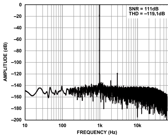
Figure 14. FFT, Median Mode, Sinc5 Filter, -0.25 dBFS
