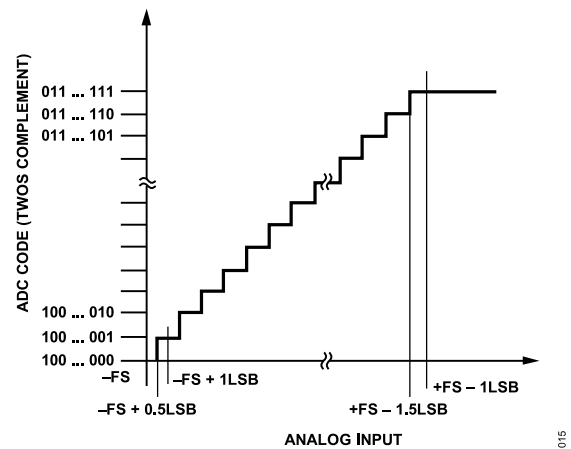
Figure 61. ADC Ideal Transfer Functions (FS is Full-Scale)
