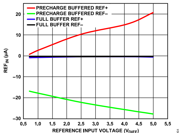
Figure 68. Reference Input Current ( REF_{IN} ) vs. Reference Input Voltage, Precharge Buffered REF+ and REF- and Full Buffer REF+ and REF-
