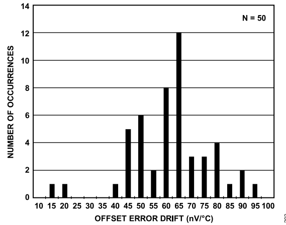
Figure 32. Offset Error Drift, Fast Mode
