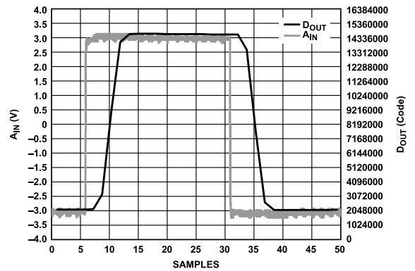
Figure 39. Step Response ( A_{IN} and D_{OUT} ) vs. Samples, Sinc5 Filter
