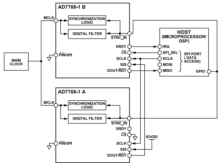
Figure 82. Daisy-Chaining Multiple AD7768-1 Devices
