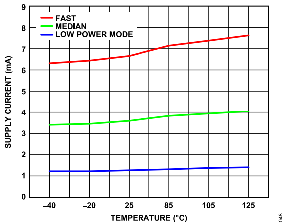
Figure 48. Supply Current vs. Temperature, AVDD1
