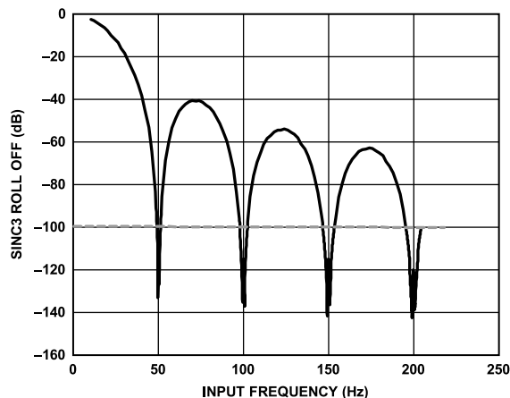
Figure 72. Sinc3 Filter Frequency Response Showing 50 Hz Rejection, 50 Hz ODR, \times 163,840 Decimation
