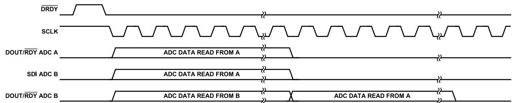
Figure 83. Data Output Format When Devices Daisy-Chained ( \overline{\text{PIN}} Control Mode Only)
