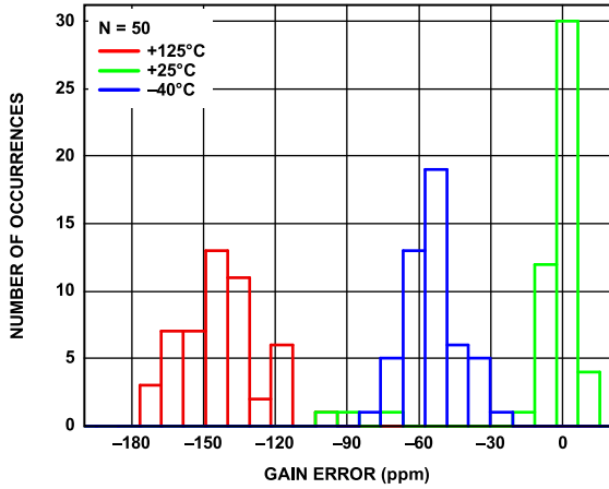
Figure 34. Gain Error Distribution, Reference Buffers On
