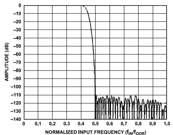
Figure 73. Low Ripple FIR Filter Frequency Response
