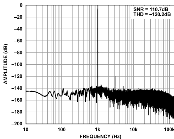
Figure 13. FFT, Fast Mode, Sinc5 Filter, -0.25 dBFS
