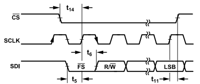
Figure 3. SPI Write Timing Diagram
