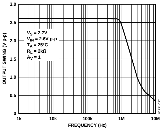
Figure 38. Closed-Loop Output Voltage Swing vs. Frequency (FPBW)
