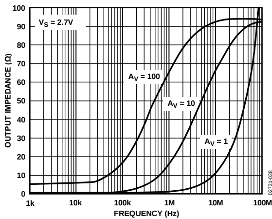
Figure 39. Output Impedance vs. Frequency
