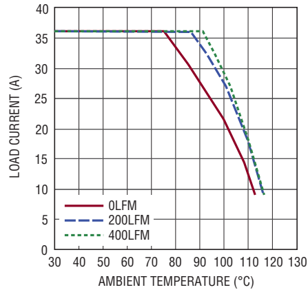
Figure 24. 5V to 1.5V Derating Curve, BGA Heat Sink
