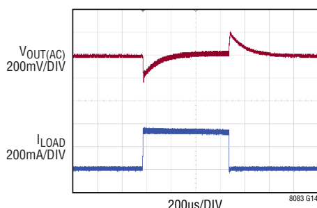
Transient Response from 12V IN to 12V OUT
