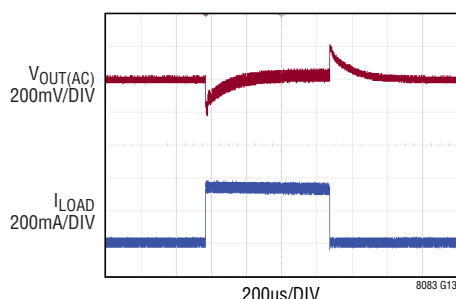
Transient Response from 6V IN to 12V OUT
