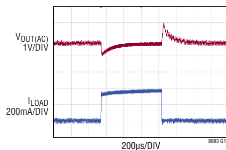
Transient Response from 36V IN to 36V OUT
