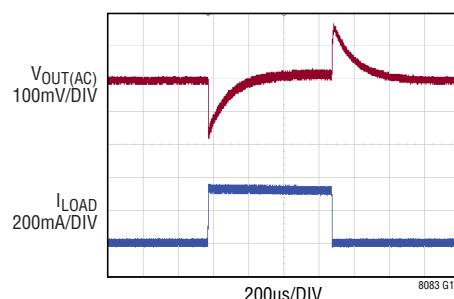
Transient Response from 24V IN to 12V OUT
