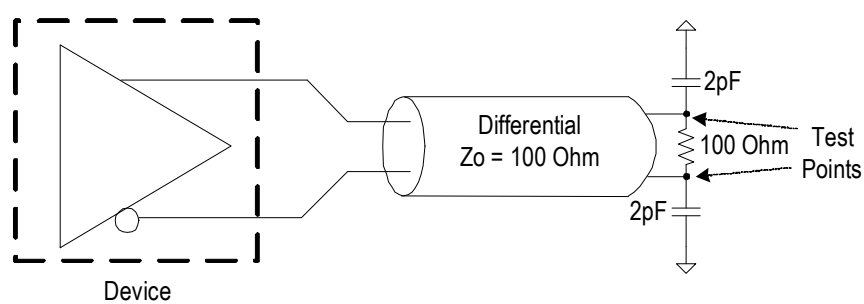
Figure 4. LVDS Test Load
