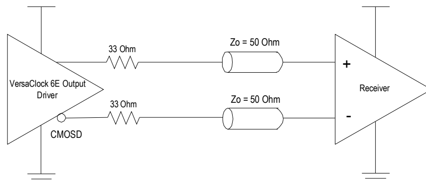
Figure 22. LVCNOS Termination
