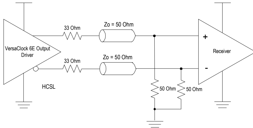
Figure 21. HCSSL Source Terminated
