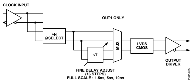
Figure 24. Analog Delay Block
