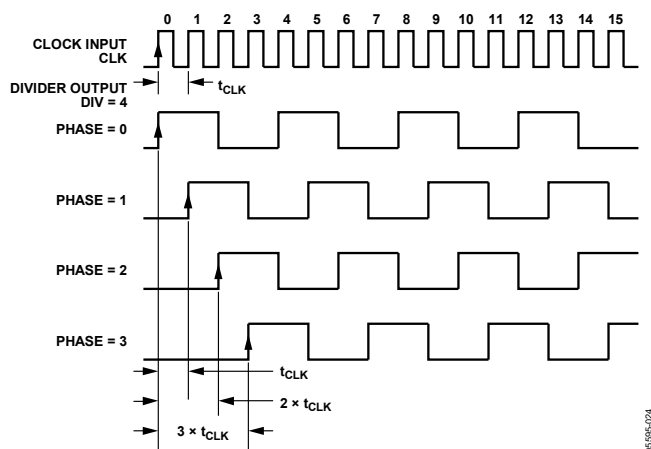
Figure 23. Phase Offset—Divider Set for Divide = 4, Phase Set from 0 to 2
